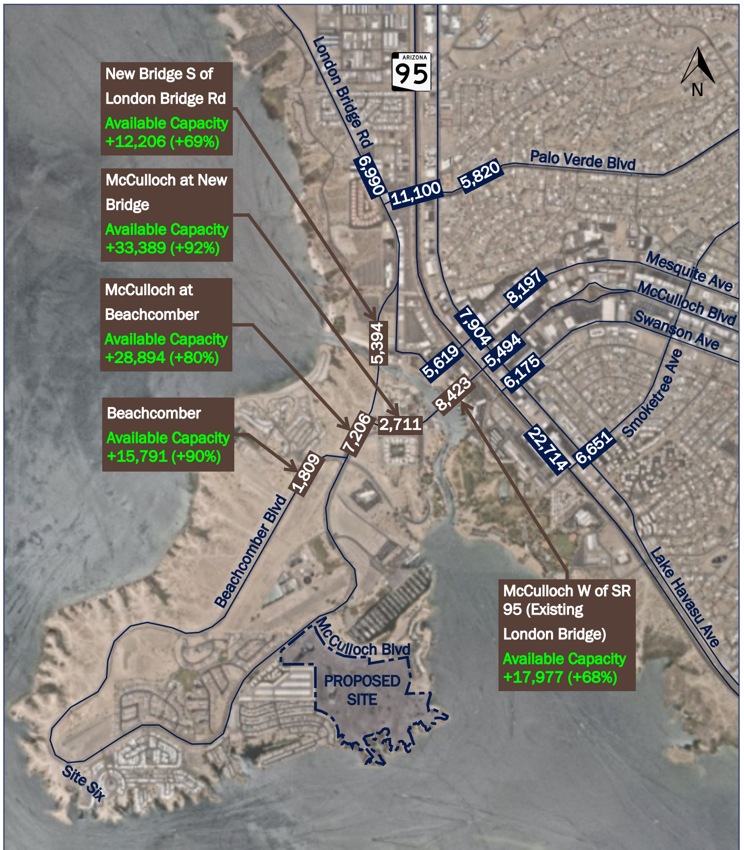
Figure 7 | Year 2030 Daily Traffic Volumes (LHC/ADOT Feasibility Study)
