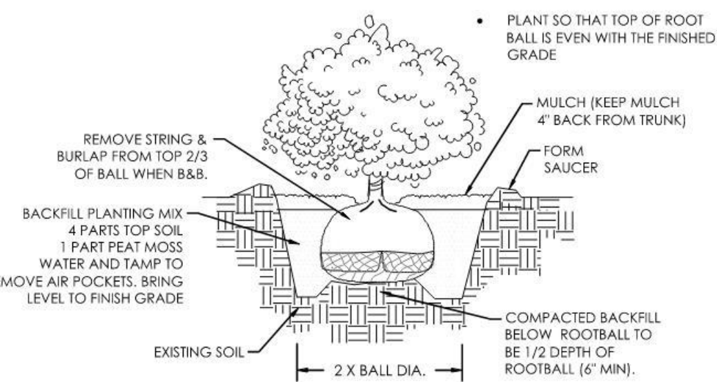
B SHRUB PLANTING NOT TO SCALE
