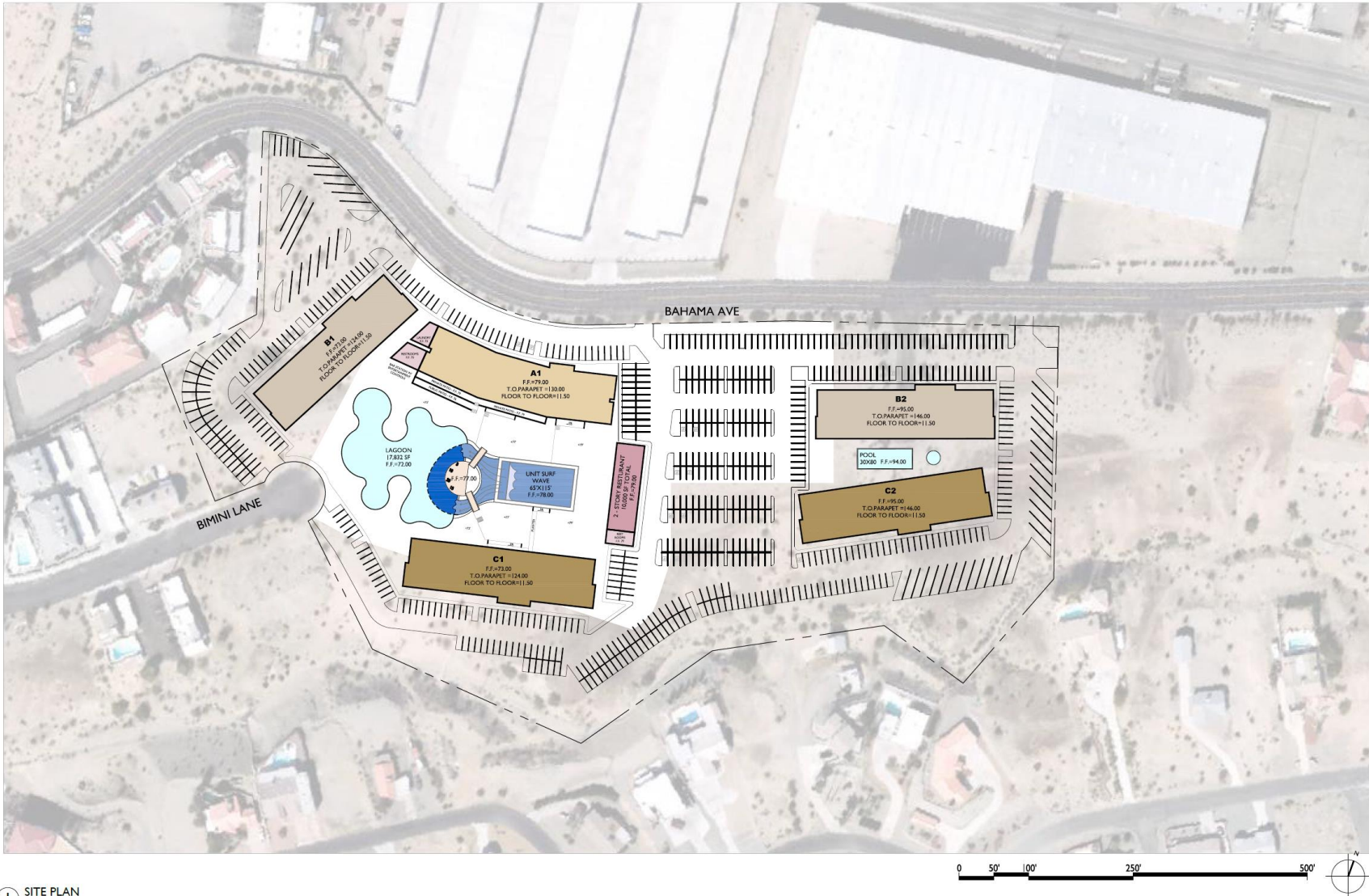
1 SITE PLAN 1/64" = 1'-0"
