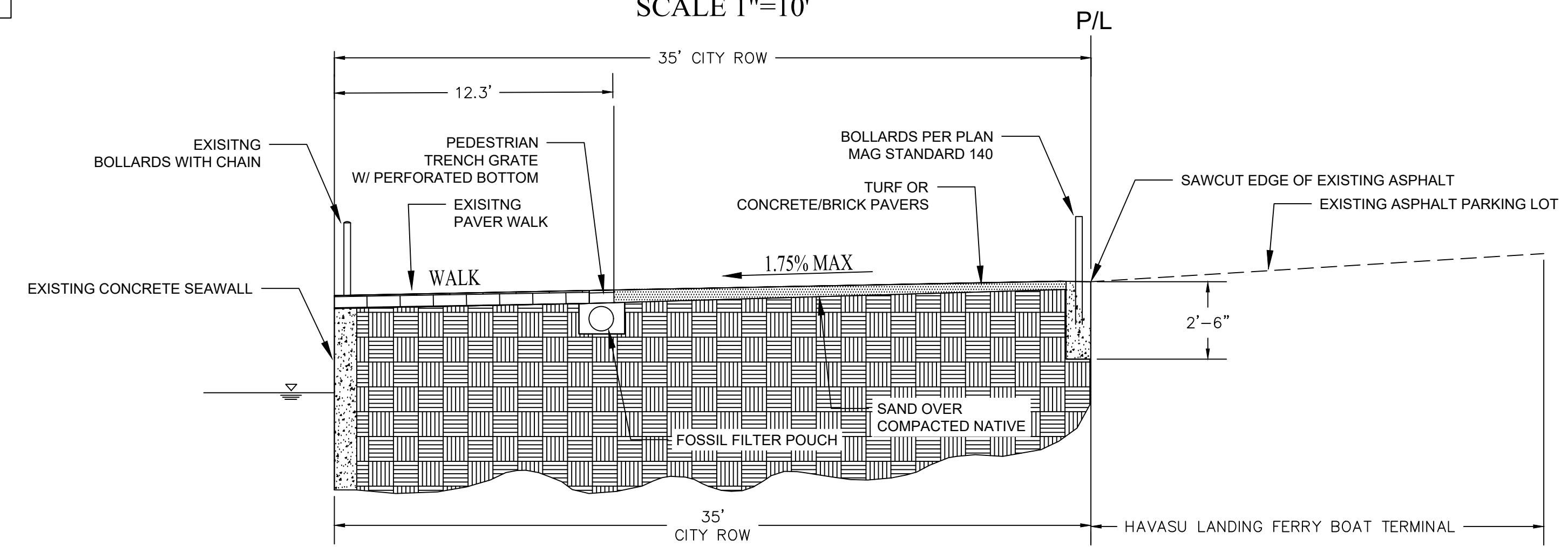
TYPICAL SECTION A-A NO SCALE
